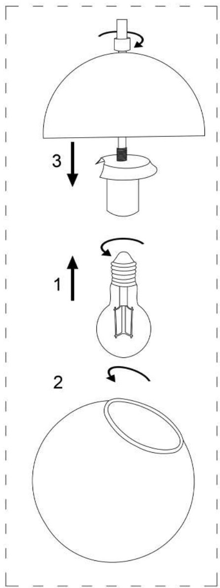
ASSEMBLY DETAIL
