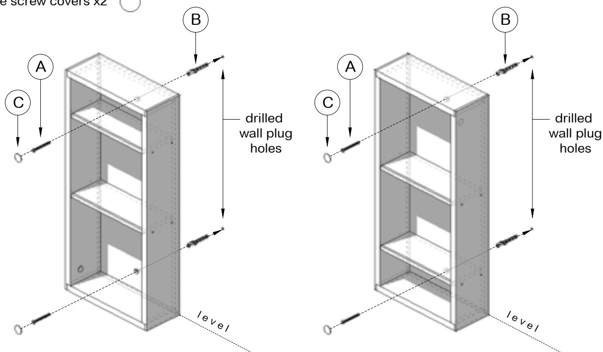
Either way installation
